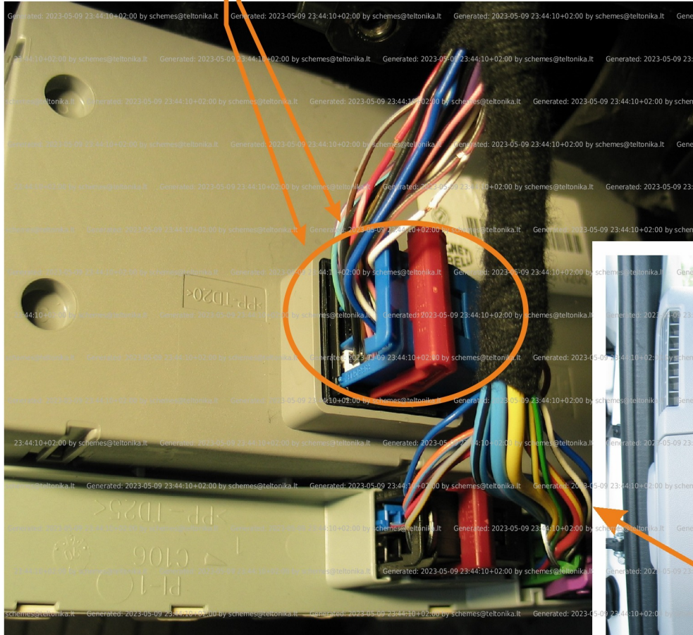
CONTROLLER MODULE (BACK)
